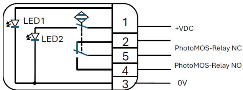
Connection plan
